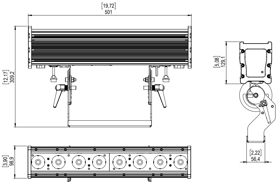
FLARE XLR 1x8 shown with yoke
