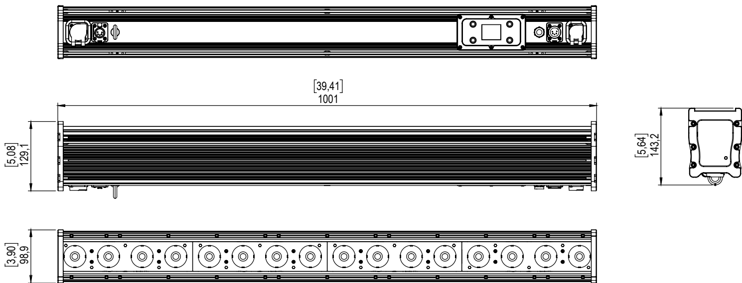
FLARE XLR 1x16 shown without yoke
